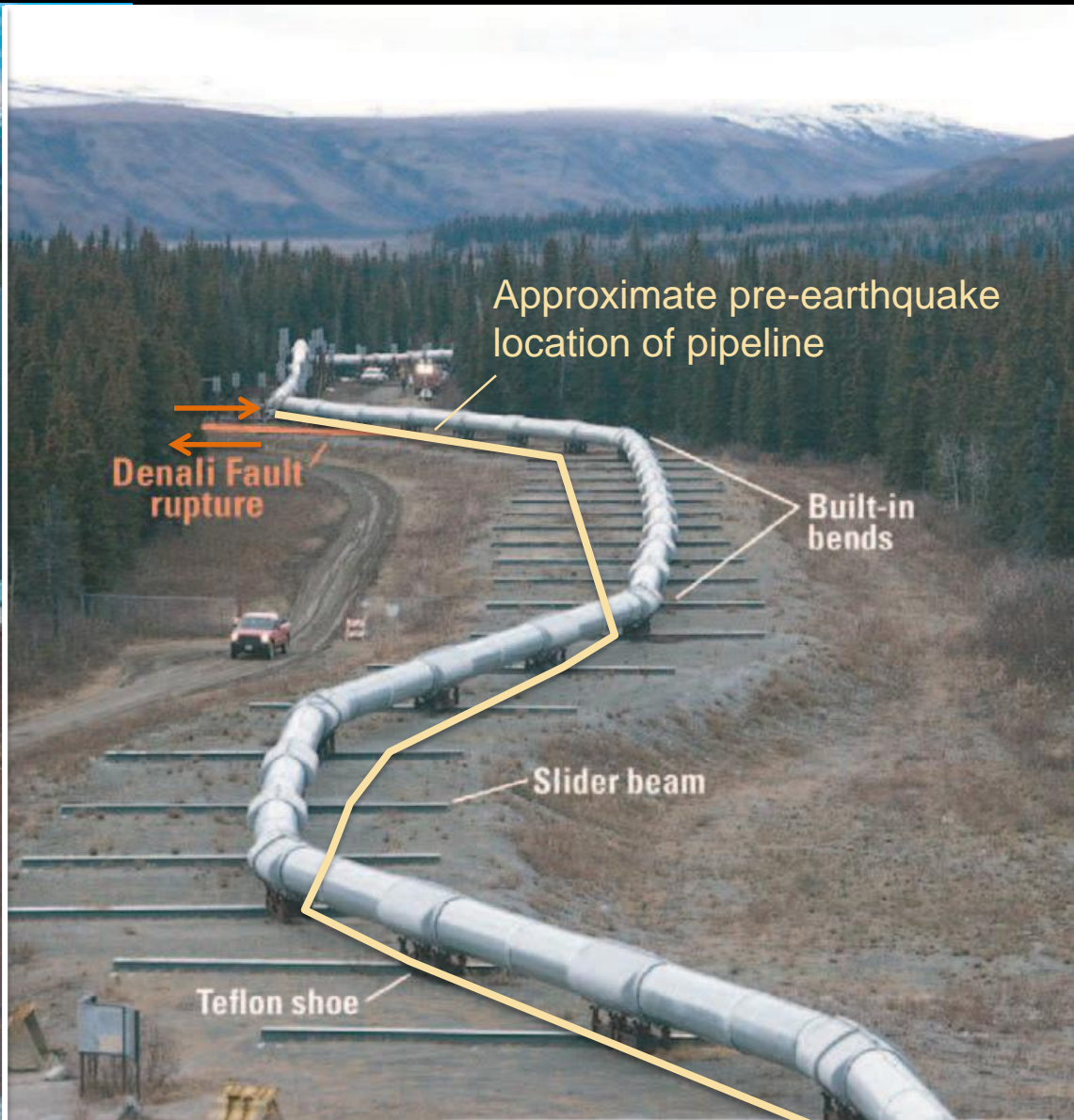
The Trans-Alaska oil pipeline survived the 2002 M7.9 Denali Fault earthquake. Pipeline design accommodated 14 feet of horizontal and 2.5 feet of vertical motion.
